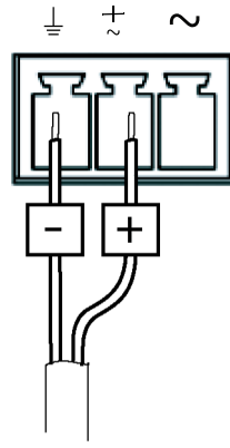
DC power input 8-28 V DC, max 10 W
